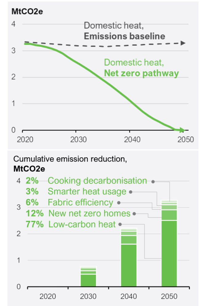
Figure 19: Decarbonisation pathway for homes in Wales and the contribution of emissions reduction measures 5
